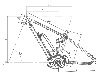
E-JAB FS 27.5
