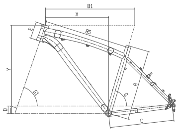
KUMA 27.5" V-BRAKE
